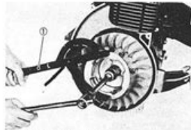
1. Primary sheave cap holding tool
