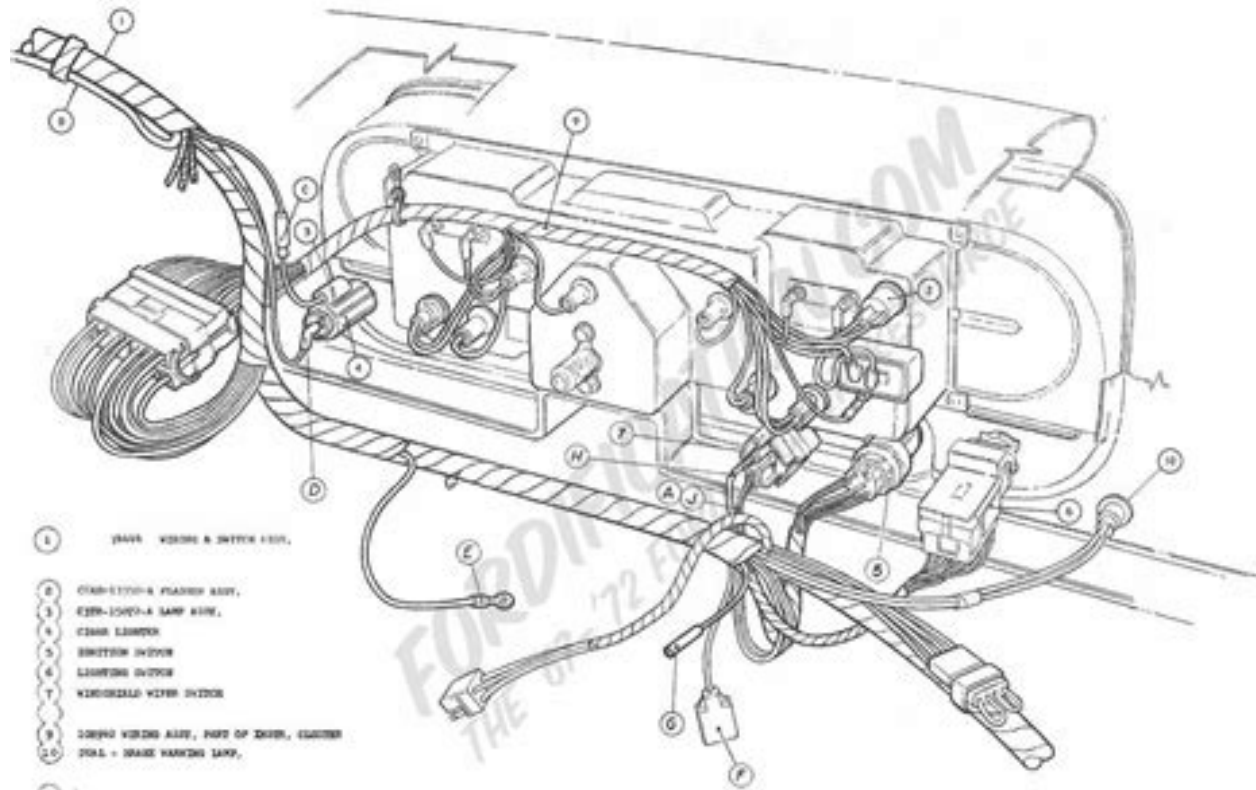
F-100 THRU F-350 INSTRUMENT PANEL MODELS 81 AND 85
